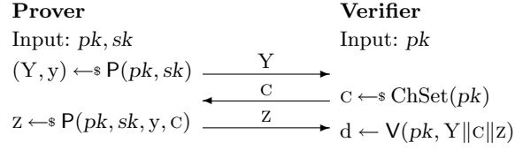
Fig. 2. \Sigma -protocol. Keys pk and sk are produced using key-generation algorithm \mathcal{K} .
