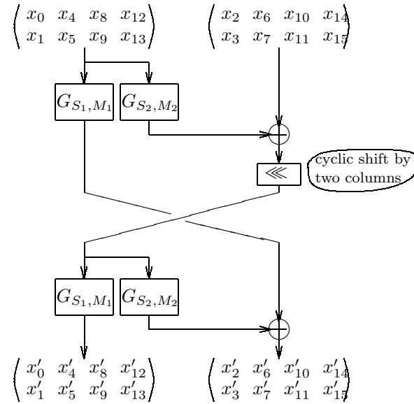
Fig. 2. The round function, F
