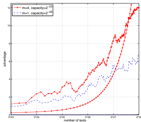
(e) Empirical and theoretical advantage for \chi^2 for m = 1 and m = 4
