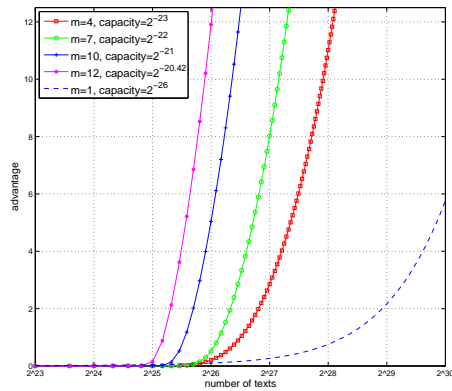
(c) Theoretical advantage for LLR-method
