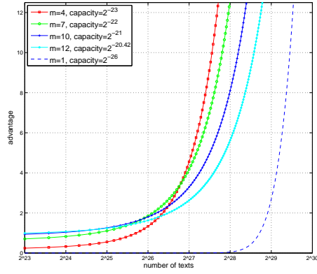
(a) Theoretical advantage for \chi^2 -method
