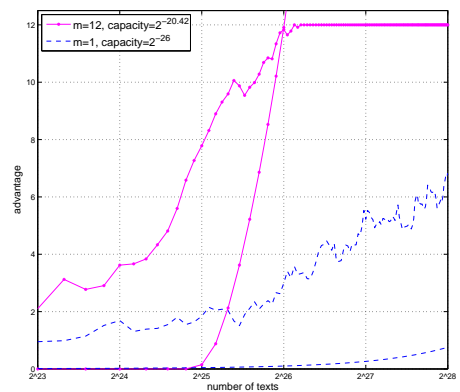
(f) Empirical and theoretical advantage for LLR for m = 1 and m = 12
