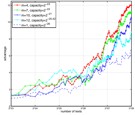
(b) Empirical advantage for \chi^2 -method
